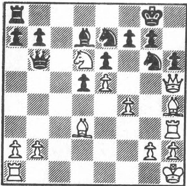
101 After 21...h6
